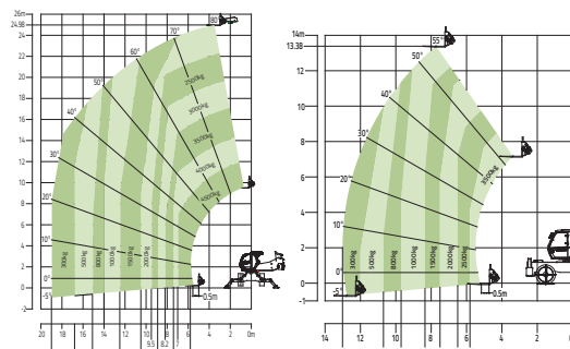
ZTH4525R作业曲线
