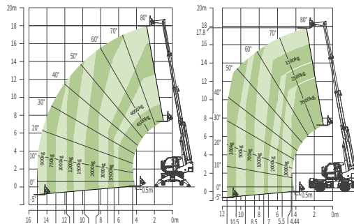
ZTH4518R作业曲线
